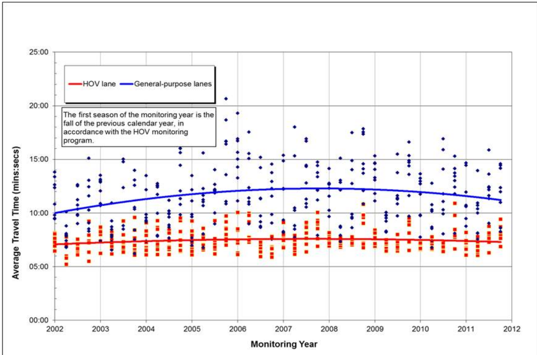
FIGURE 3 Southeast Expressway Travel Times: Southbound Travel Lanes, PM Peak Period, 2002-11
