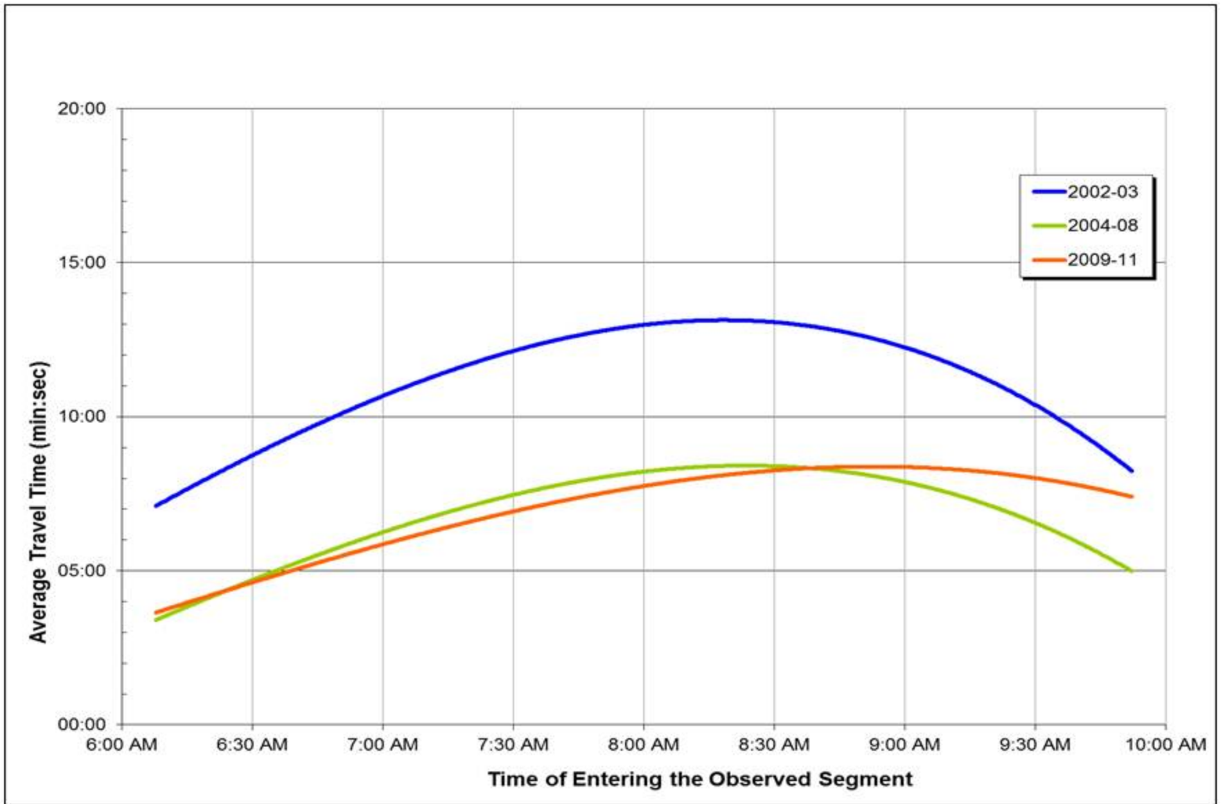
FIGURE 5 I-93 North Travel Times: Southbound General-Purpose Lanes, AM Peak Period, 2002-11
