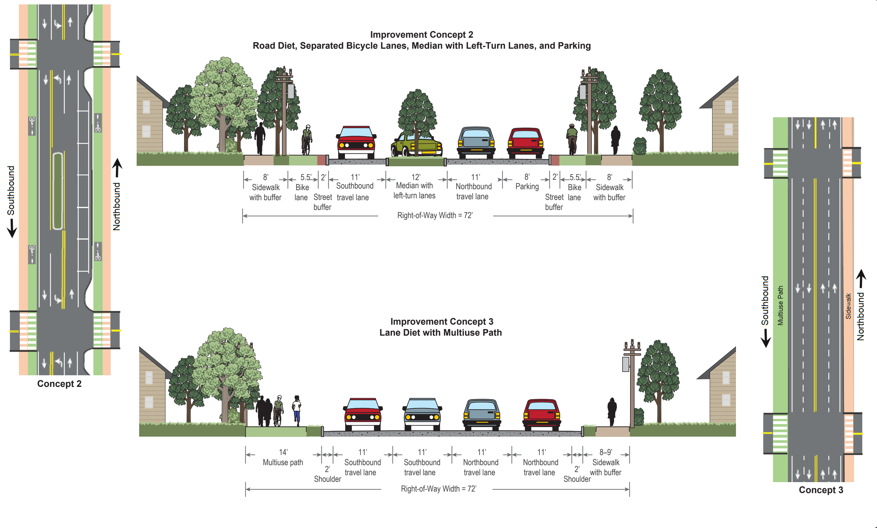
Figure 21 Reedsdale Road: Long-Term Improvements Concepts 2 and 3
