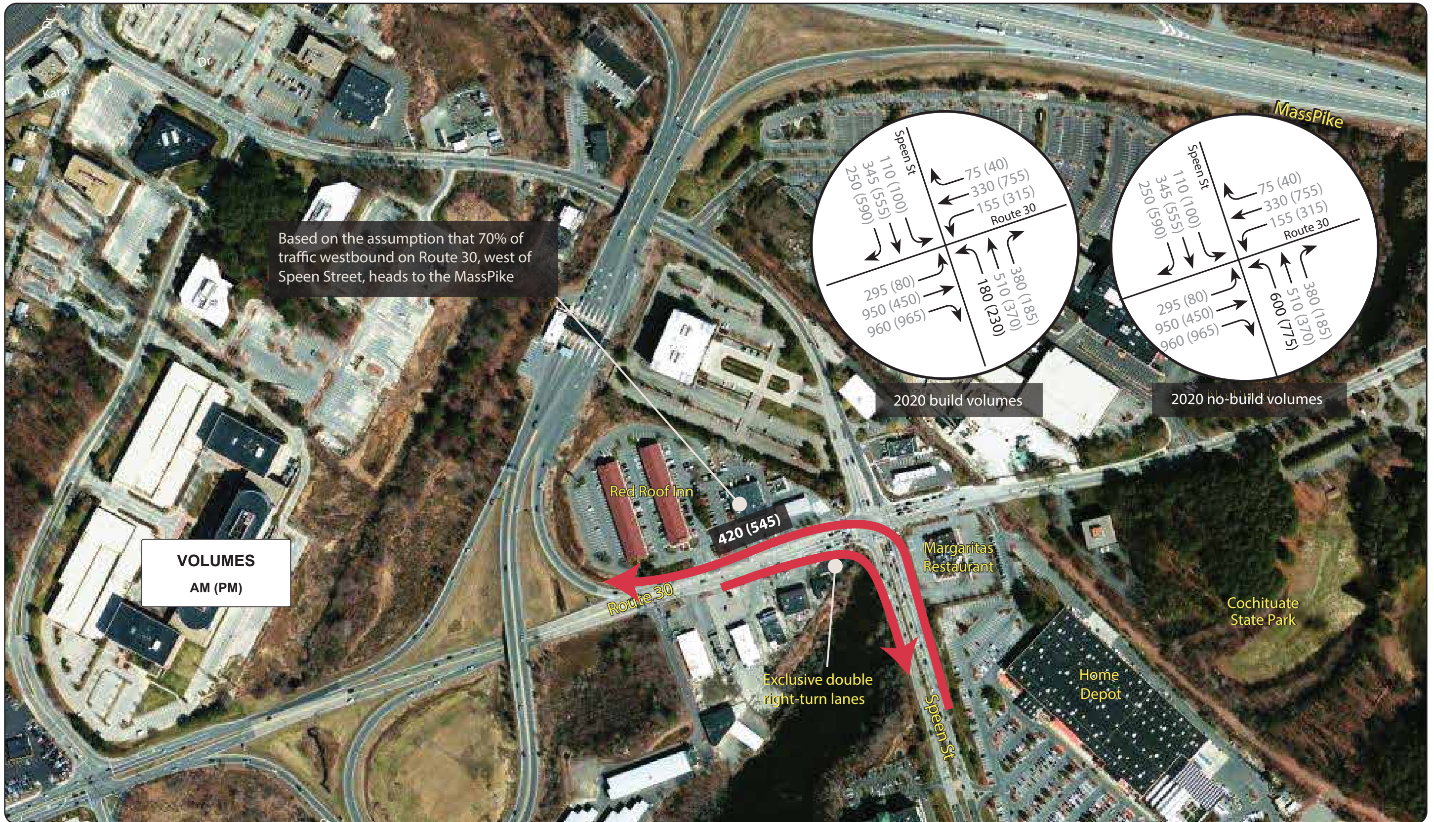
FIGURE 12 Concept 2: Grade-Separated Spenn Street Northbound Left Turn and Route 30 Eastbound Exclusive Double Right Turn Lanes
