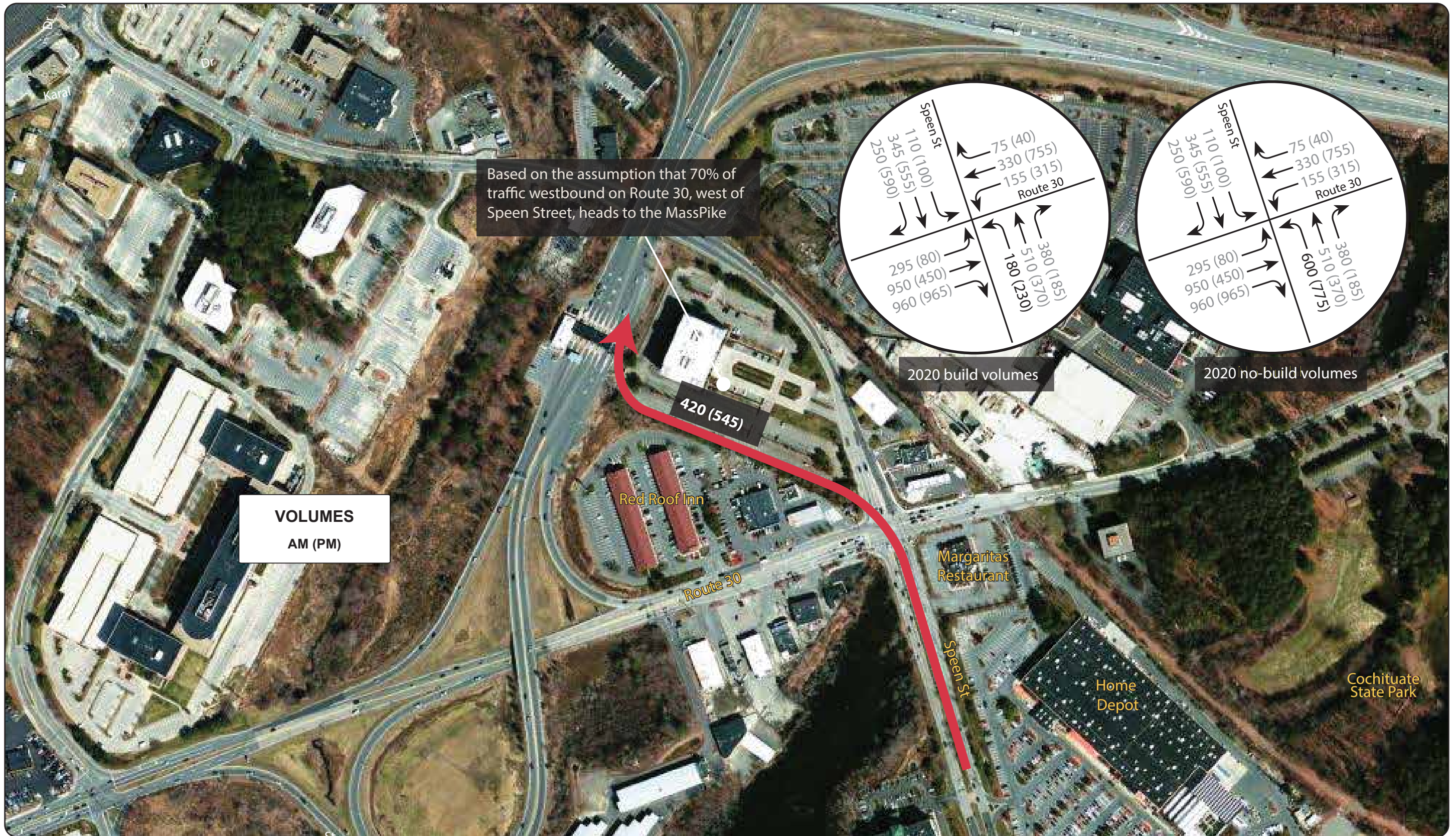
FIGURE 13 Concept 3: Grade-Separated Median Left Turn from Spenn Street Northbound to MassPike (Eastbound and Westbound)
