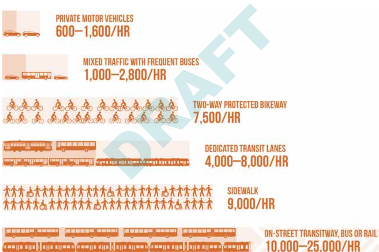
Figure 6-1 Overall Person Throughput Capacity of a Typical Lane by Mode
