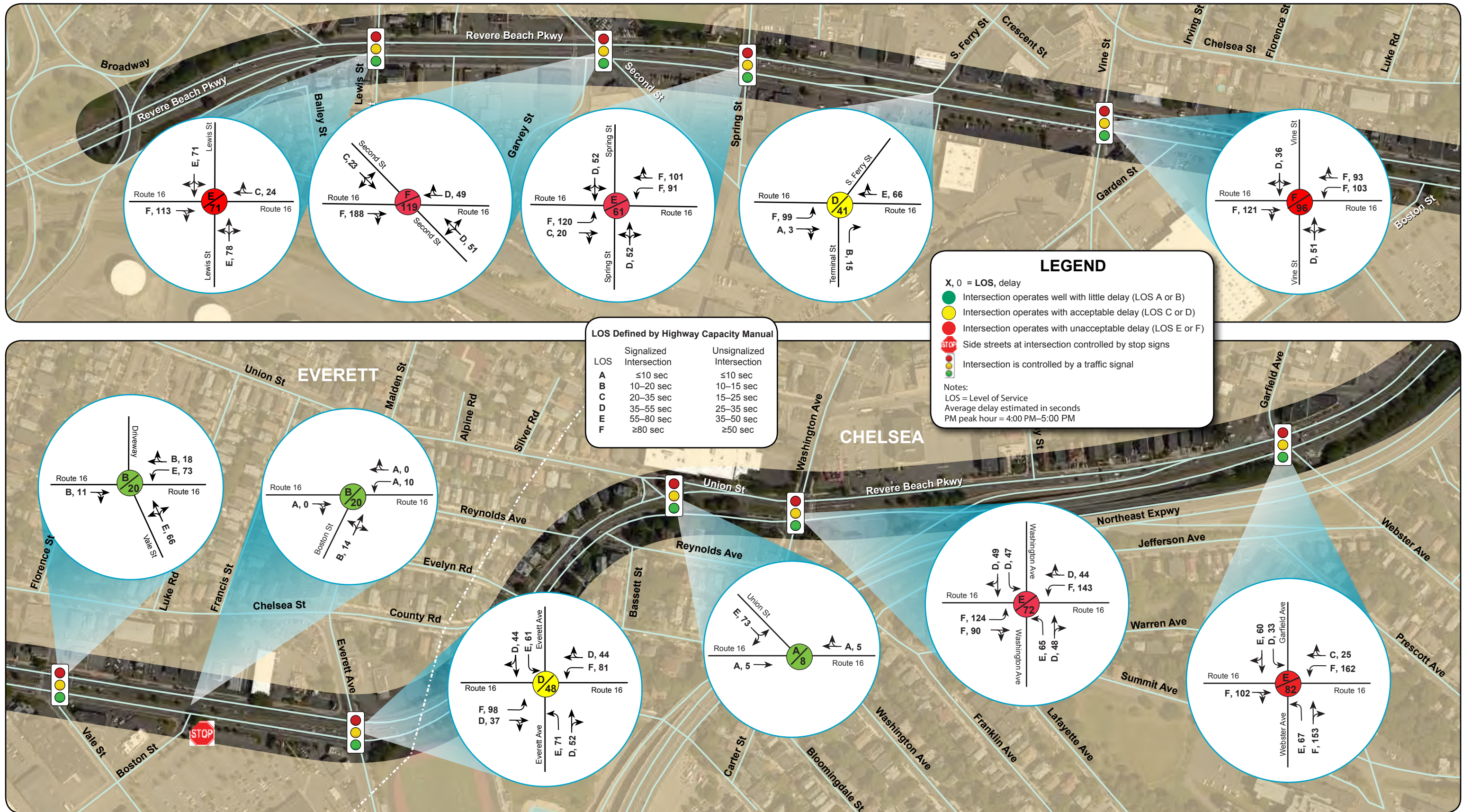
Figure 16 Weekday PM Peak-Hour Level of Service and Delay
